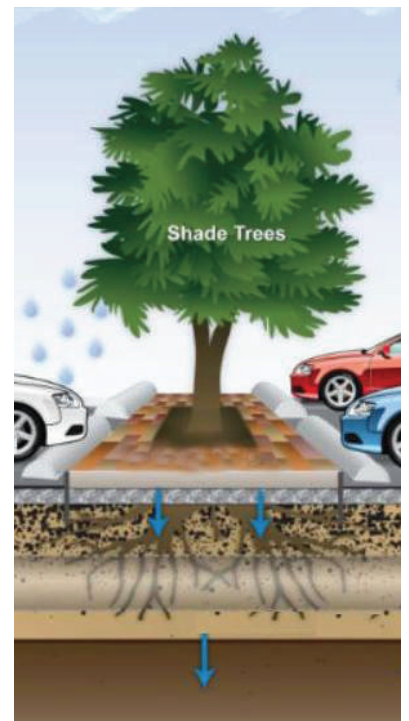
Tree Trench Illustration
