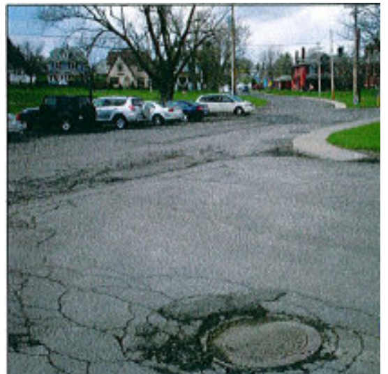
Town Hall Parking Lot before Porous Pavement Was Installed
