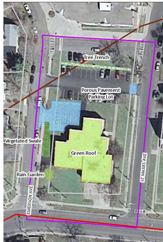
Green Infrastructure Site Plan for Hazard Library
