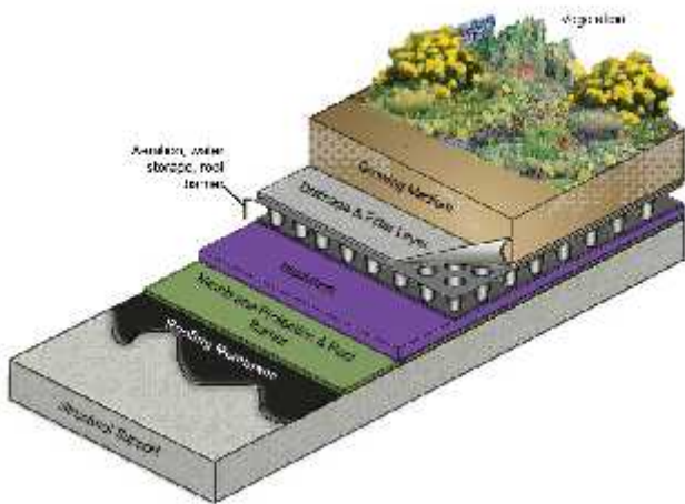
Layers of a Green Roof System
